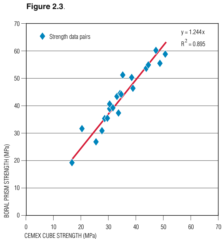
FIGURE 2.3 Correlation of mortar strength data
