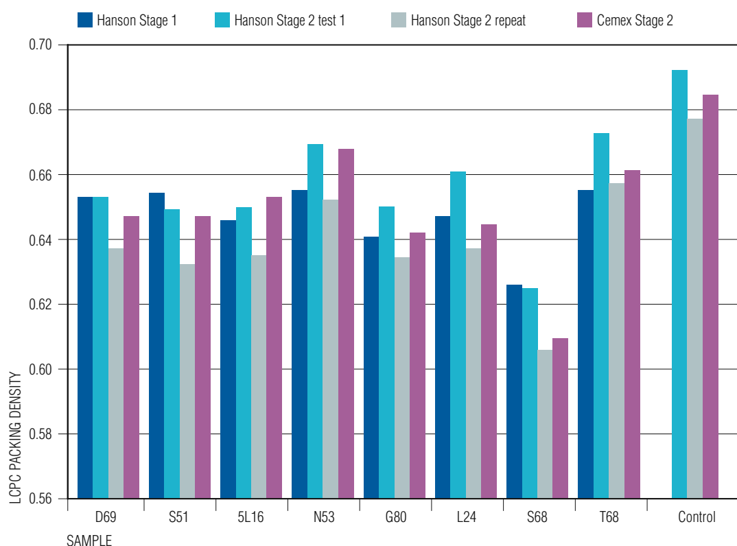
FIGURE 1.1 LCPC packing density test results
