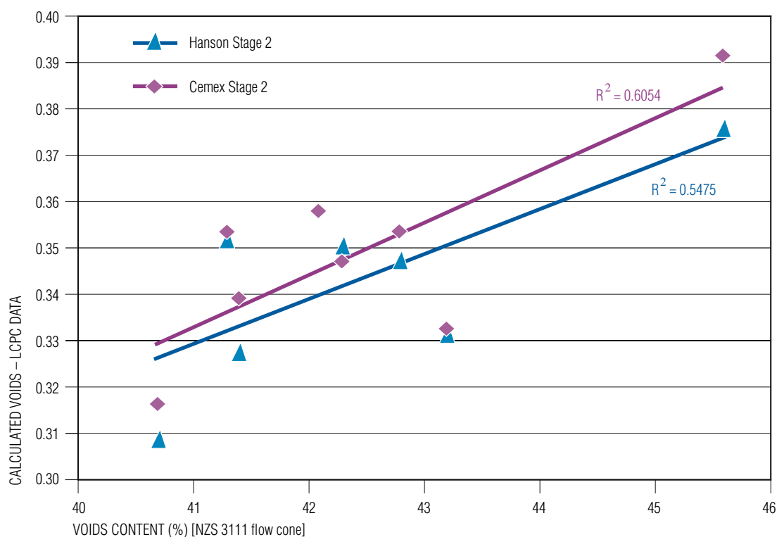
FIGURE 1.2 Correlation between measured voids and LCPC packing density
