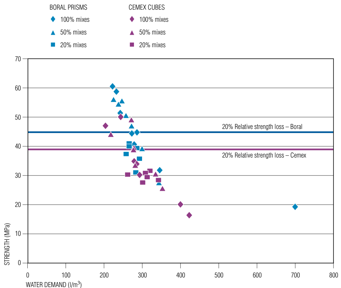
FIGURE 2.4 28-day strength results
