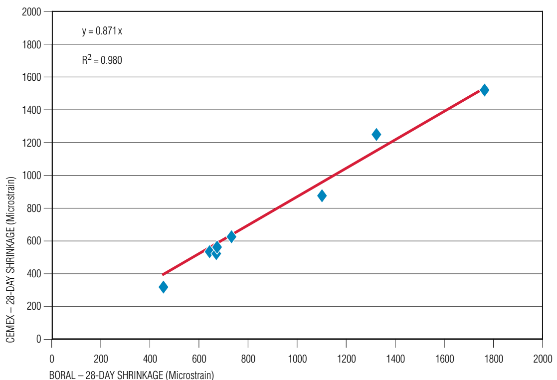
FIGURE 2.6 Shrinkage comparison (microstrain)
